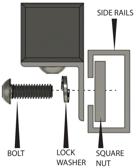
Santacruz Adapter assembly
